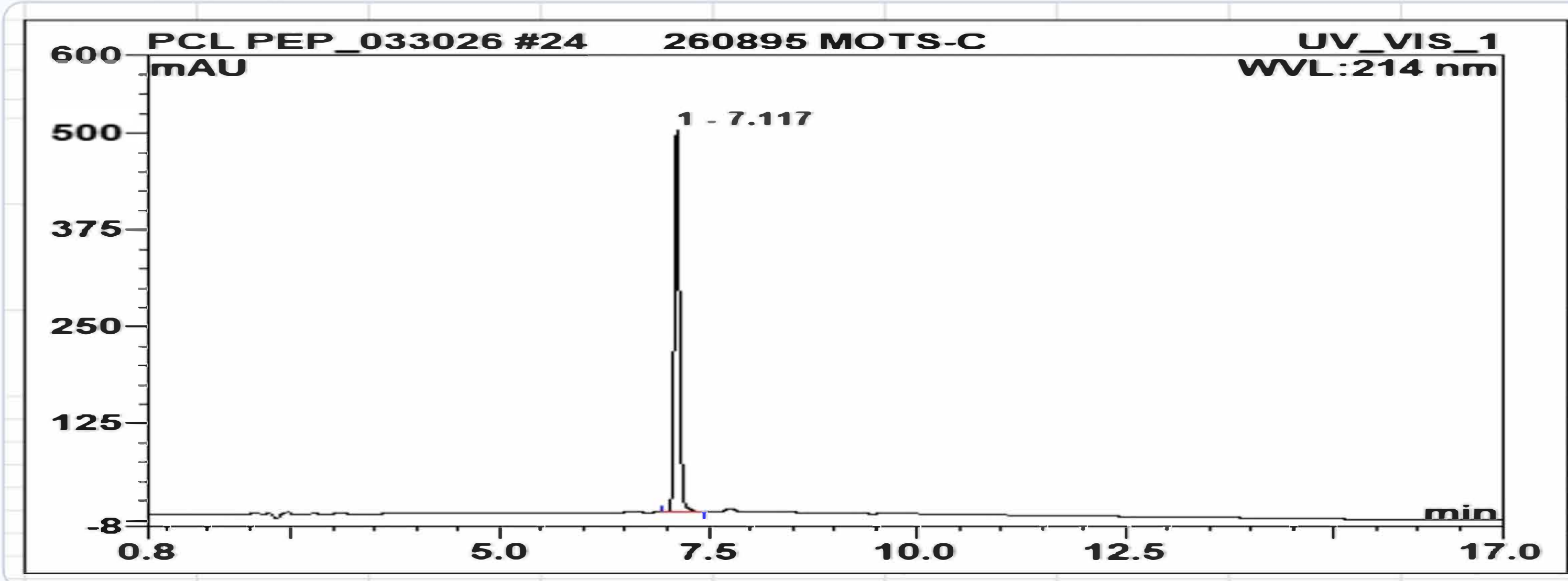
HPLC Chromatogram (Retention Time: 7.117 min)
