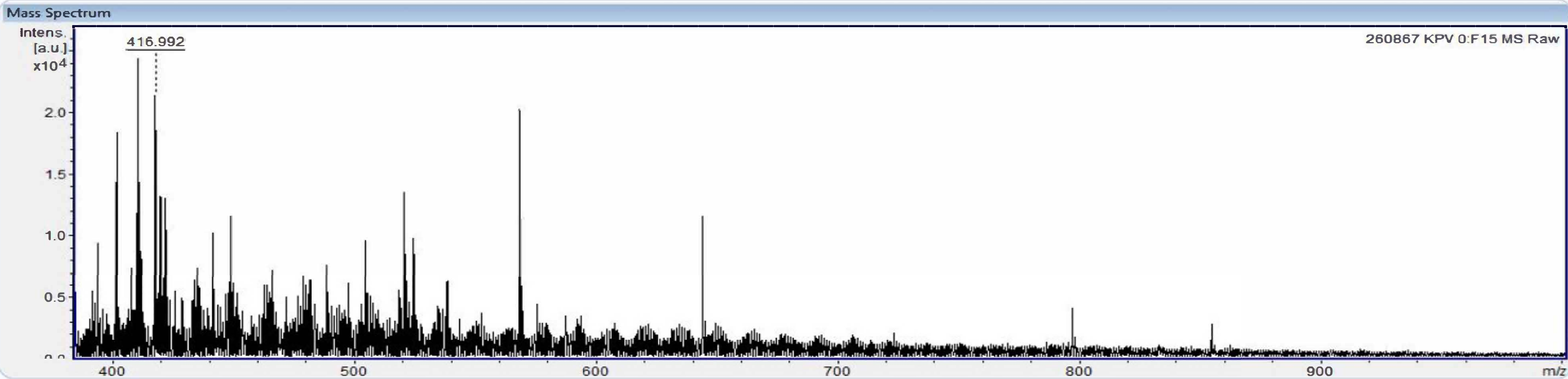
Mass Spectrum (MALDI-MS)
