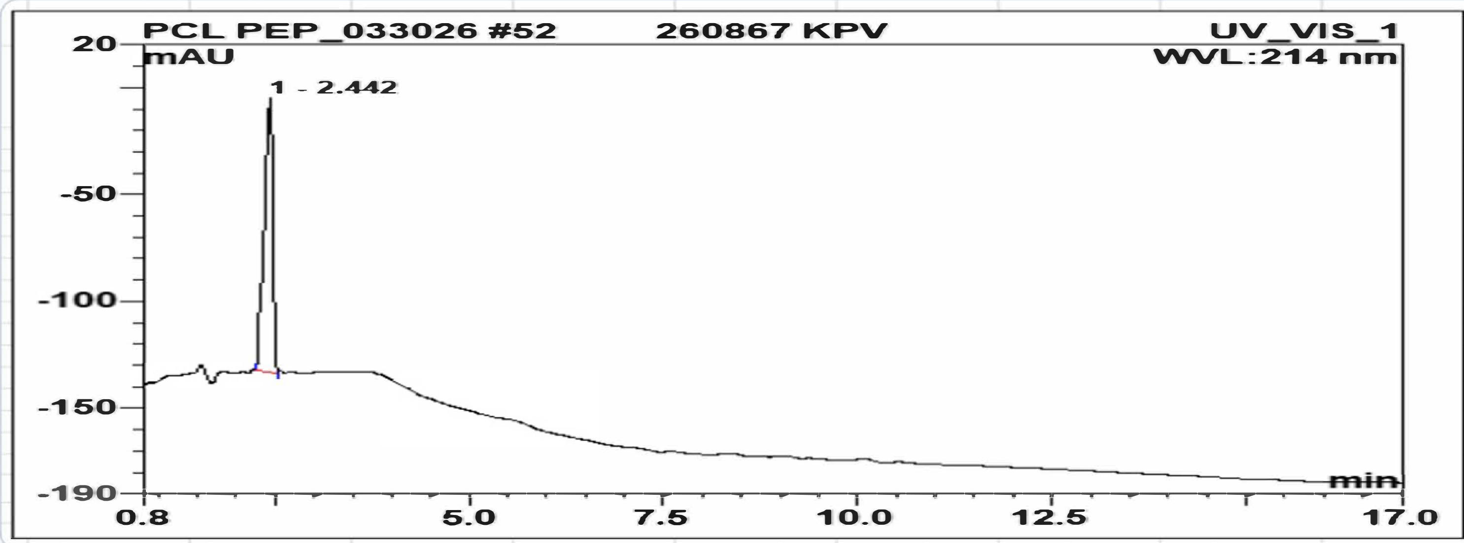
HPLC Chromatogram (Retention Time: 2.442 min)
